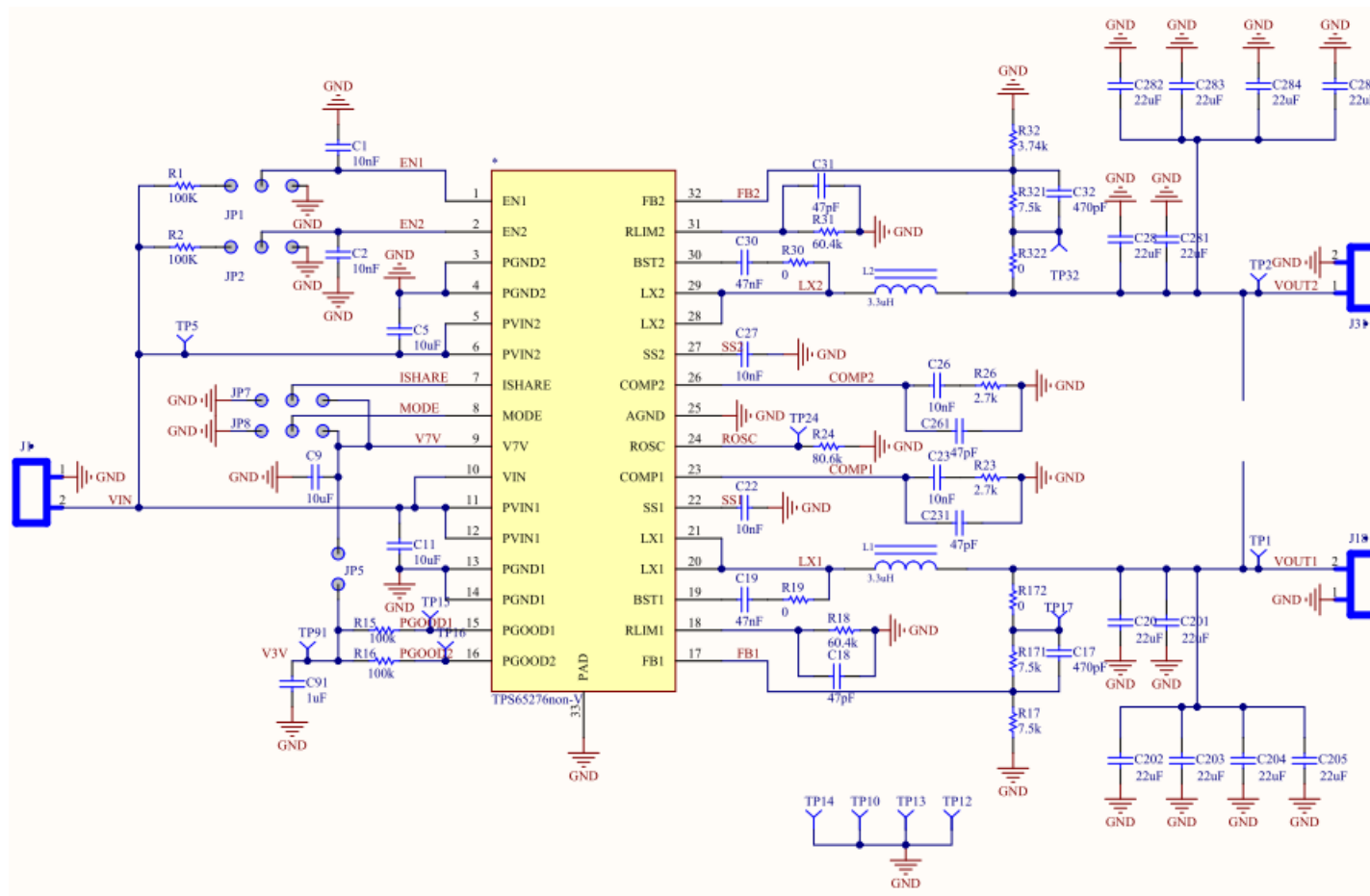
Figure 1. TPS65276 Schematic
